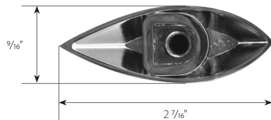
Screw hole: 1/4" - 20
